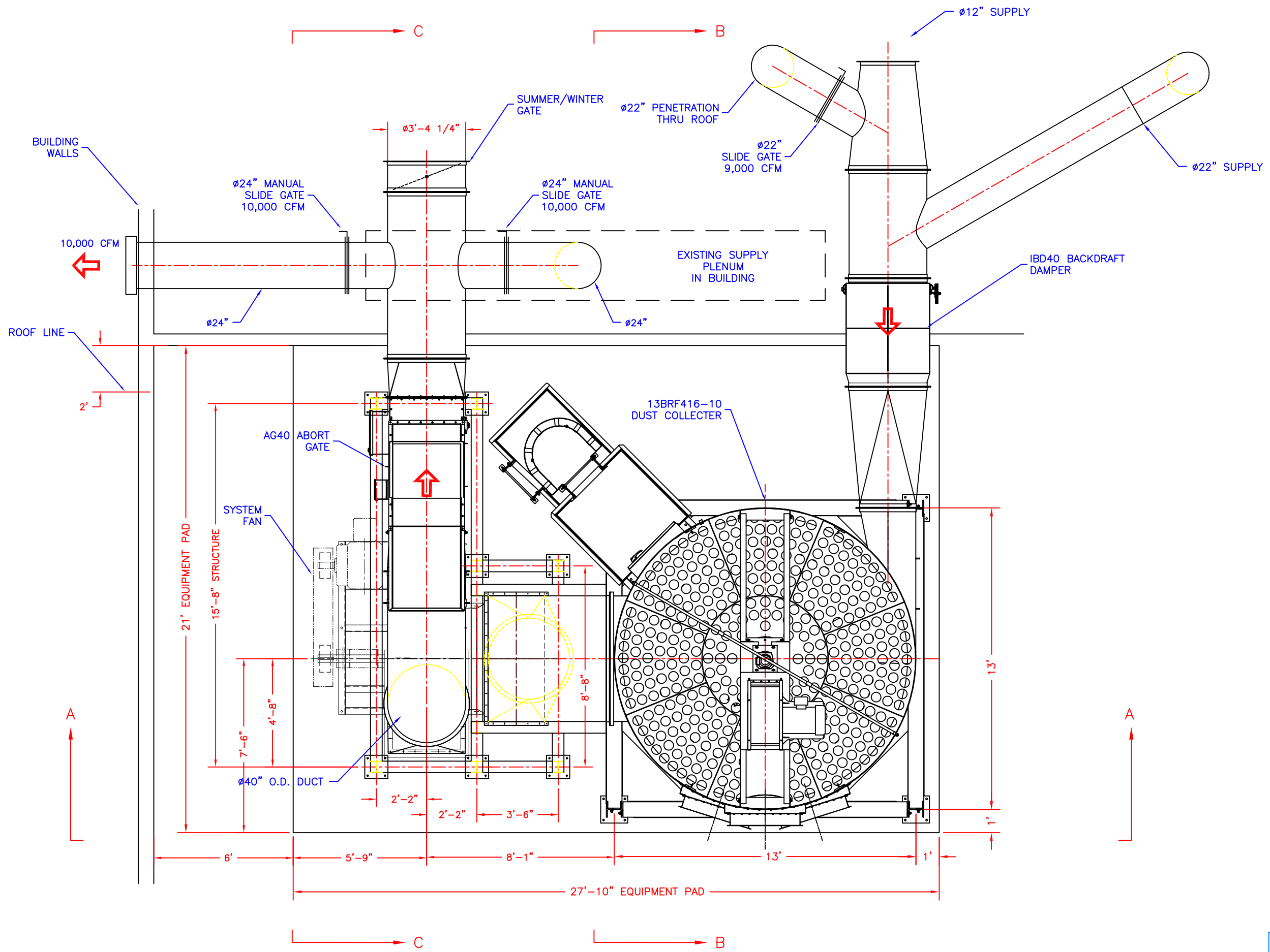
PLAN VIEW
